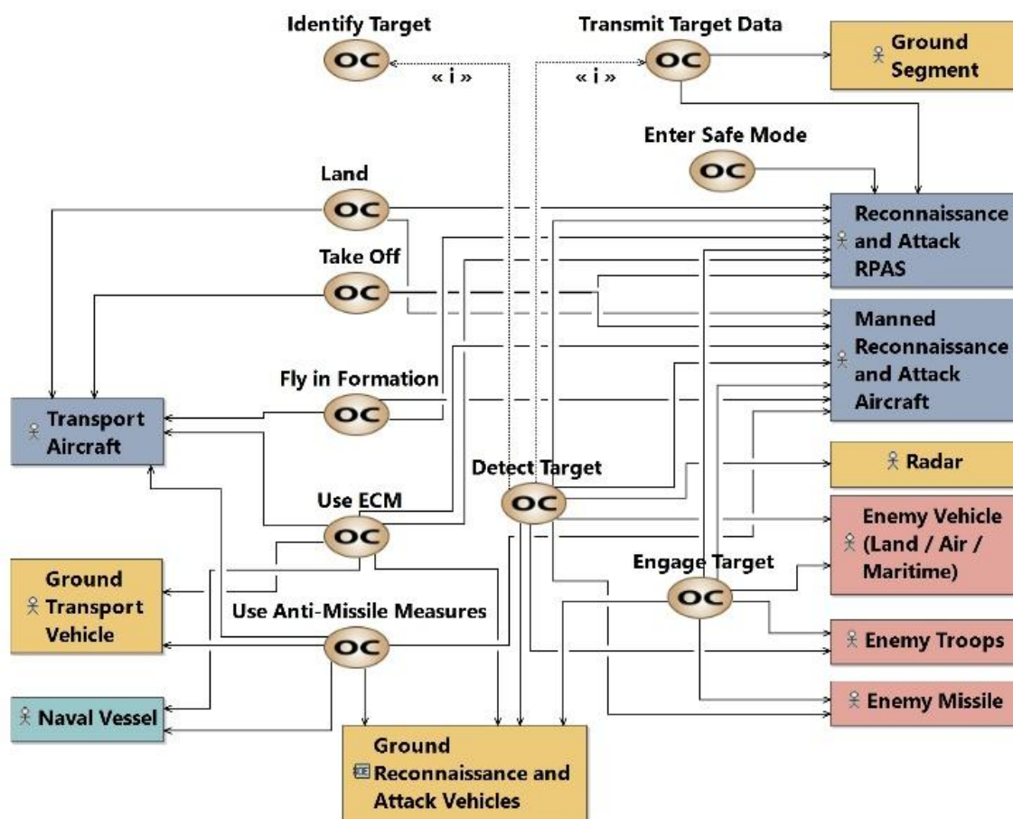
Fig. 4. Use Case Diagram for the Attack RPAS.
