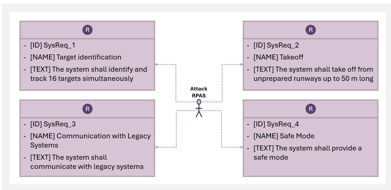
Fig. 5. Extract of the System Requirements diagram.
